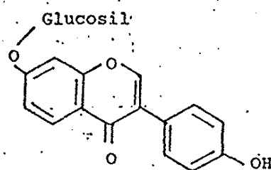
[IV] Daidzin
