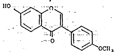
[VII] Formononetin
