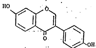
[III] Daidzein
